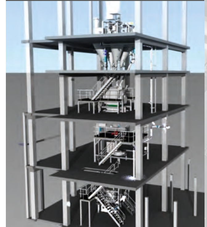
An overview of the gravity mixing line for which the cleaning times were measured
